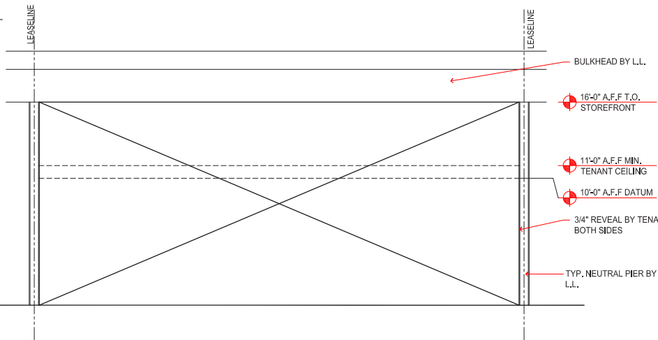
TYPICAL ZONE 3 INTERIOR STOREFRONT ELEVATION SCALE: 1/8" = 1'-0"
