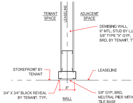
TYPICAL NEUTRAL PIER SCALE: 1/2" = 1'-0"
