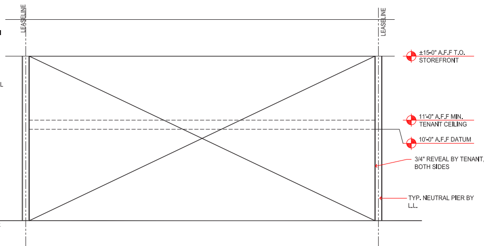
TYPICAL ZONE 5 INTERIOR STOREFRONT ELEVATION SCALE: 1/8" = 1'-0"
