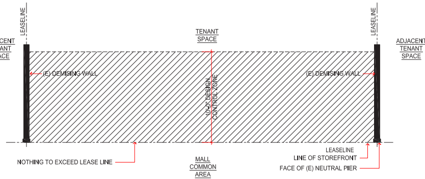
TYPICAL ZONE 1 INTERIOR STOREFRONT PARTIAL PLAN SCALE: 1/8" = 1'-0"
