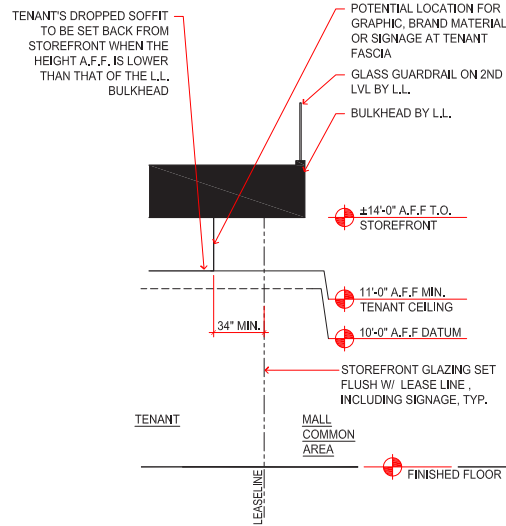
TYPICAL ZONE 1 STOREFRONT SECTION SCALE: 1/8" = 1'-0"
