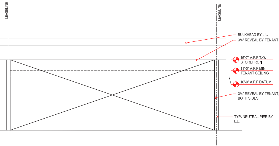
TYPICAL ZONE 4 INTERIOR STOREFRONT ELEVATION SCALE: 1/8" = 1'-0"
