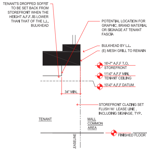
TYPICAL ZONE 4 STOREFRONT SECTION SCALE: 1/8" = 1'-0"
