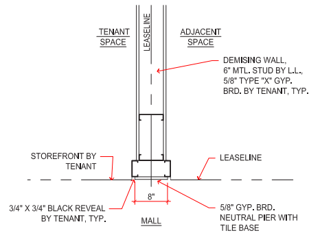
TYPICAL NEUTRAL PIER SCALE: 1/2" = 1'-0"
