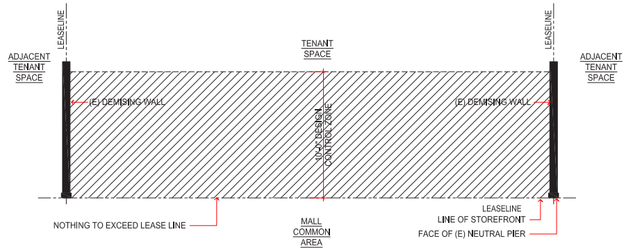
TYPICAL ZONE 4 INTERIOR STOREFRONT PARTIAL PLAN SCALE: 1/8" = 1'-0"
