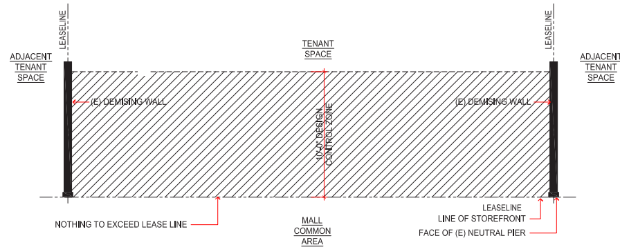
TYPICAL ZONE 3 INTERIOR STOREFRONT PARTIAL PLAN SCALE: 1/8" = 1'-0"
