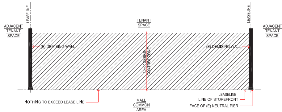
TYPICAL ZONE 5 INTERIOR STOREFRONT PARTIAL PLAN SCALE: 1/8" = 1'-0"
