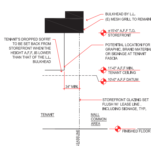
TYPICAL ZONE 5 STOREFRONT SECTION SCALE: 1/8" = 1'-0"
