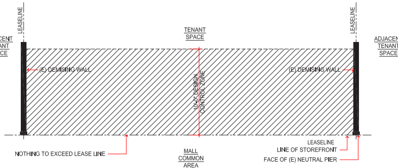
TYPICAL ZONE 2A INTERIOR STOREFRONT PARTIAL PLAN SCALE: 1/8" = 1'-0"
