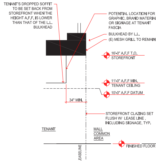
TYPICAL ZONE 3 STOREFRONT SECTION SCALE: 1/8" = 1'-0"
