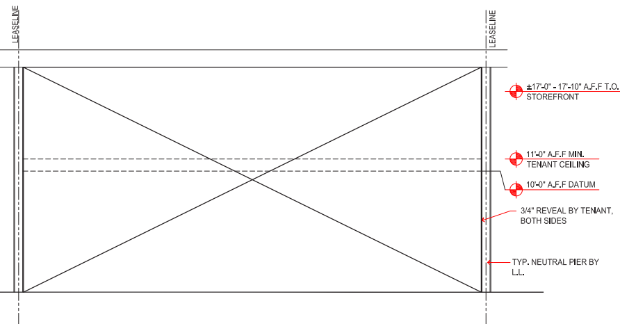
TYPICAL ZONE 2A INTERIOR STOREFRONT ELEVATION SCALE: 1/8" = 1'-0"
