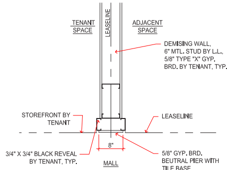
TYPICAL NEUTRAL PIER SCALE: 1/2" = 1'-0"
